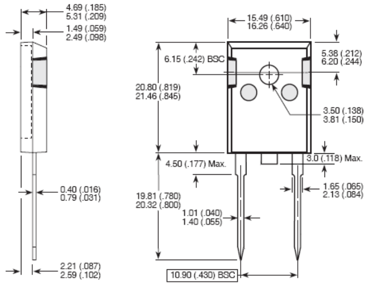
Fig8. Package Outline
