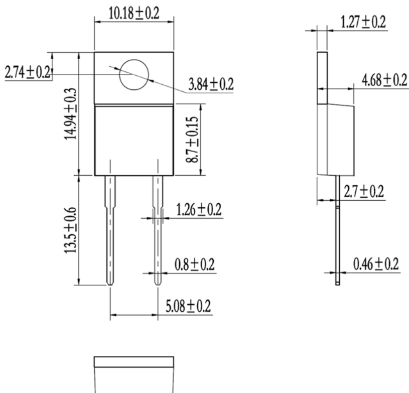
Figure 8. Package Outline
