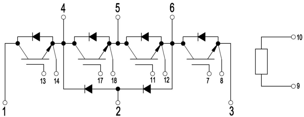
Figure 13. Circuit Diagram
