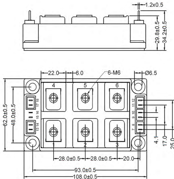
Dimensions in (mm) Figure 14. Package Outline
