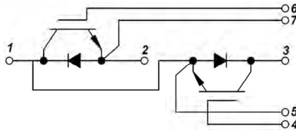
Figure 13. Circuit Diagram
