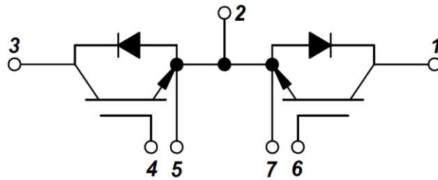
Figure 13. Circuit Diagram
