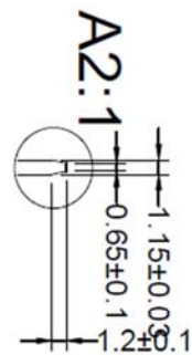
Dimensions in (mm) Figure 15. Package Outline
