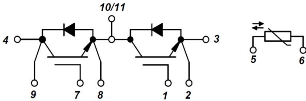
Figure 14. Circuit Diagram
