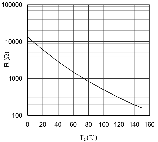
Figure 13. NTC Characteristics
