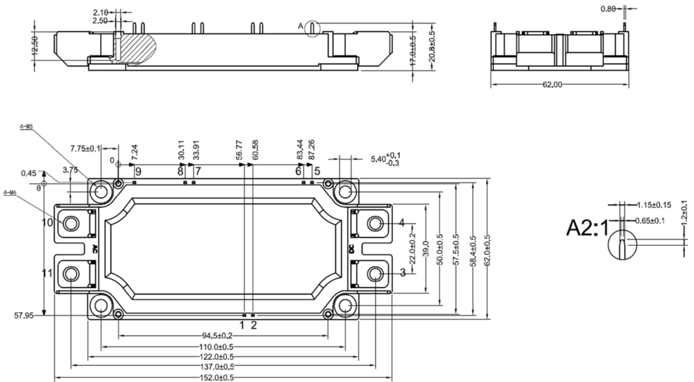
Figure 15. Package Outline
