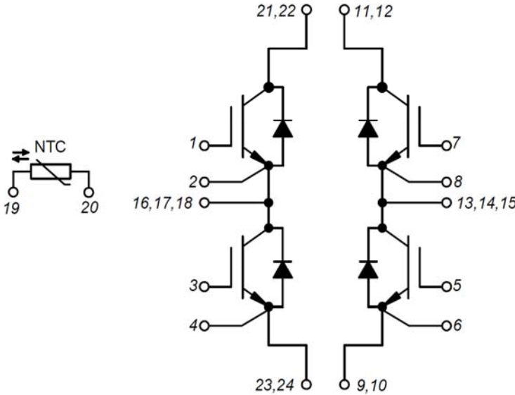
Figure 14. Circuit Diagram
