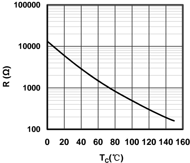
Figure 13. NTC Characteristics
