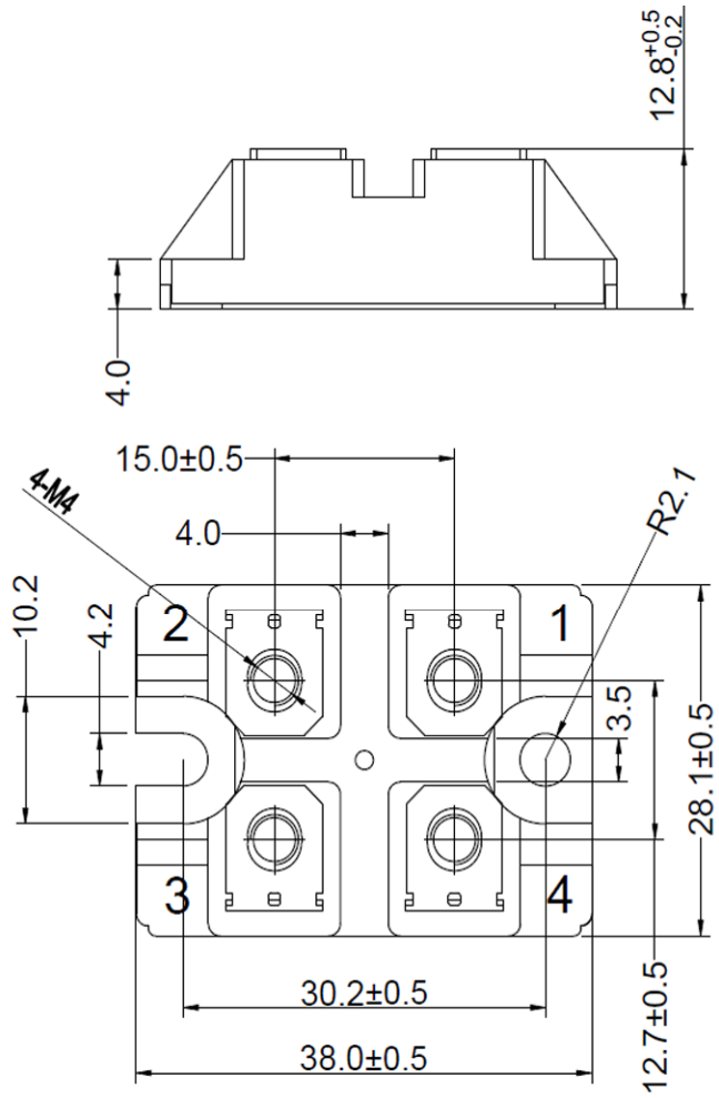
Dimensions in (mm) Figure 13. Package Outline
